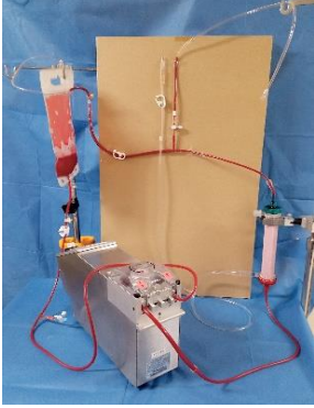
Figure 1. Photograph of test circuit
