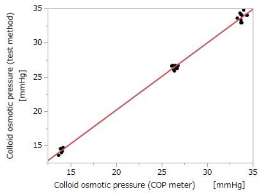
Figure 5. Correlation between COP measurements from the colloid osmometer and by the Test Method in Experiment 2
