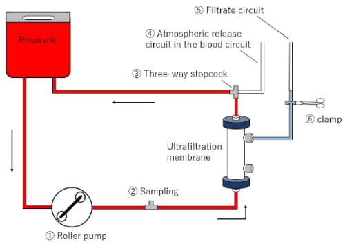
Figure 2a. Test circuit diagram (blood circulation before measurement)
