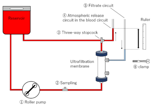
Figure 2b. Test circuit diagram (during colloid osmotic pressure measurement)
